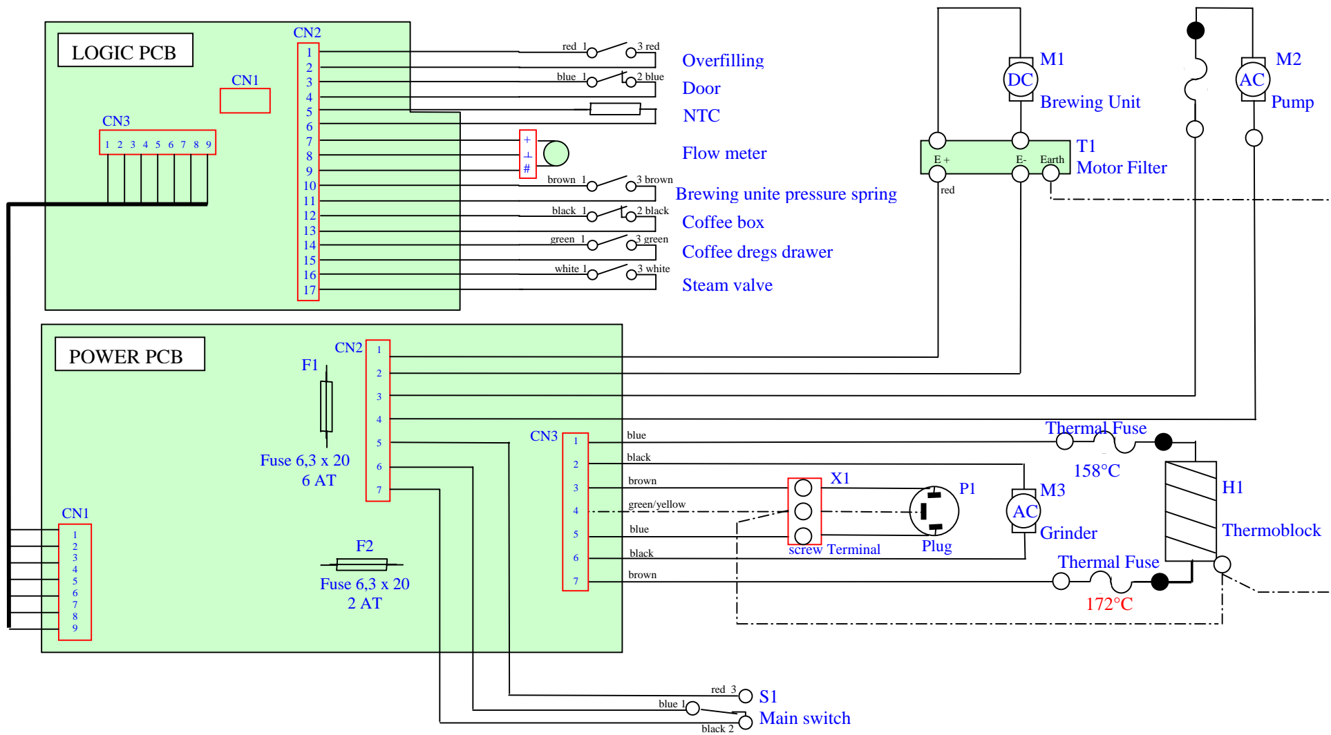
CA FAMOSA CF220/250/260 Wiring diagram 220 V – 240 V
