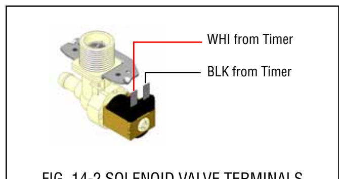
FIG. 14-2 SOLENOID VALVE TERMINALS
