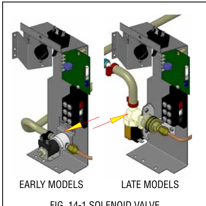
FIG. 14-1 SOLENOID VALVE
