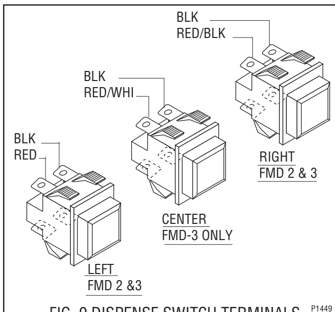
FIG. 9 DISPENSE SWITCH TERMINALS P1449
