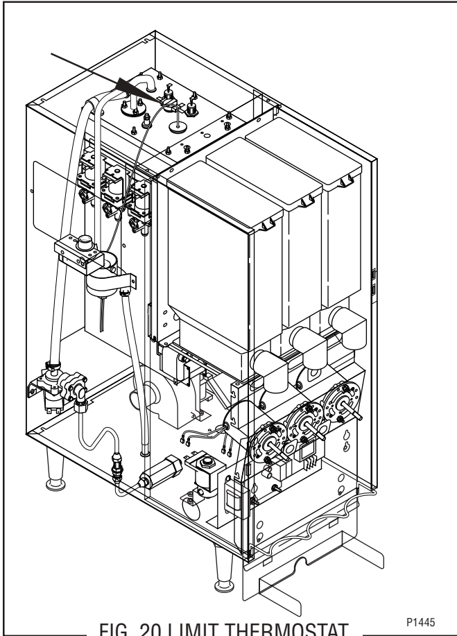
FIG. 20 LIMIT THERMOSTAT
