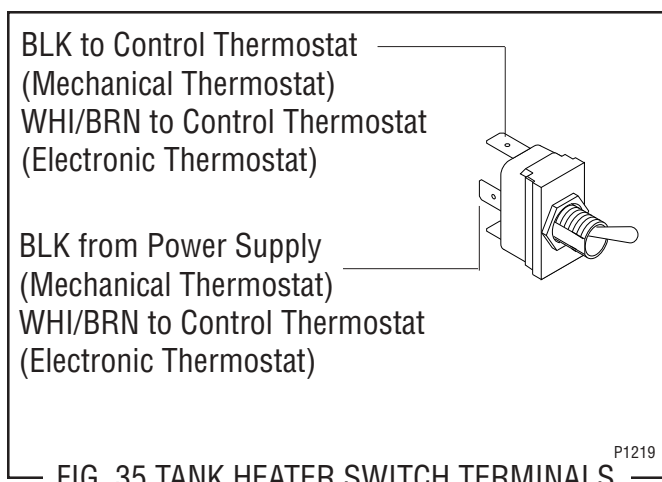
FIG. 35 TANK HEATER SWITCH TERMINALS
