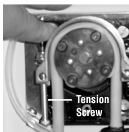
Release Spring Tension
