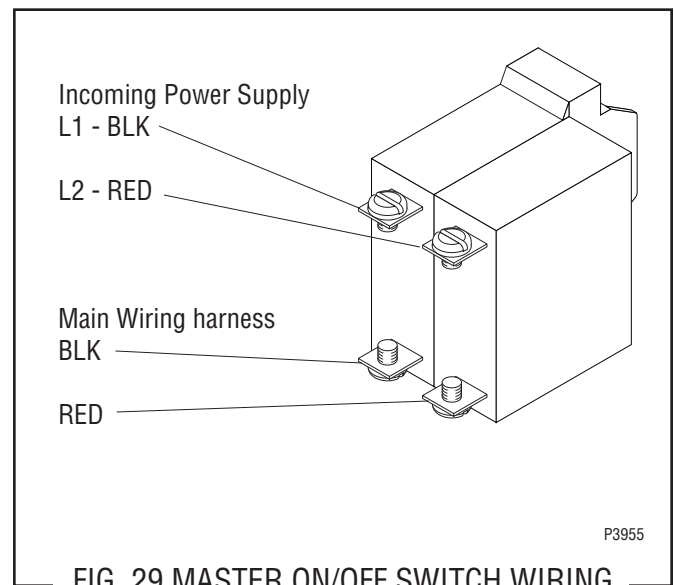
FIG. 29 MASTER ON/OFF SWITCH WIRING
