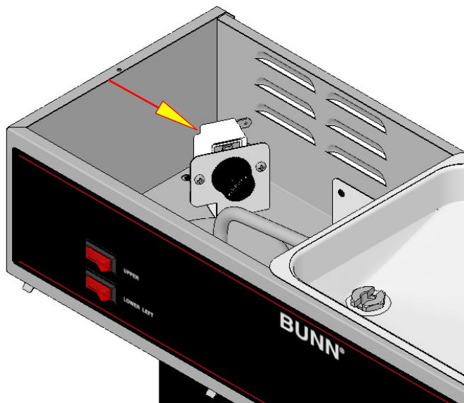
FIG. 8-1 CONTROL THERMOSTAT
